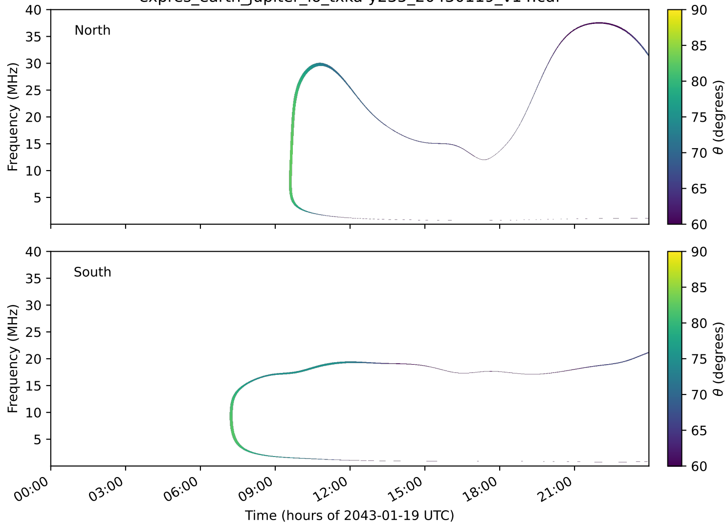
expres_earth_jupiter_io_txka-y235_20430119_v14.cdf
