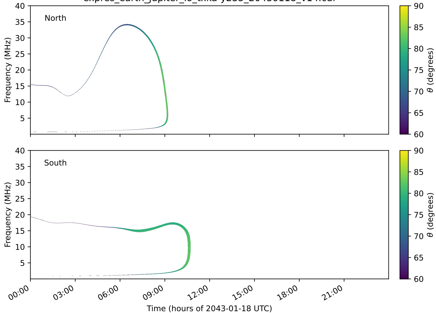
expres_earth_jupiter_io_txka-y235_20430118_v14.cdf
