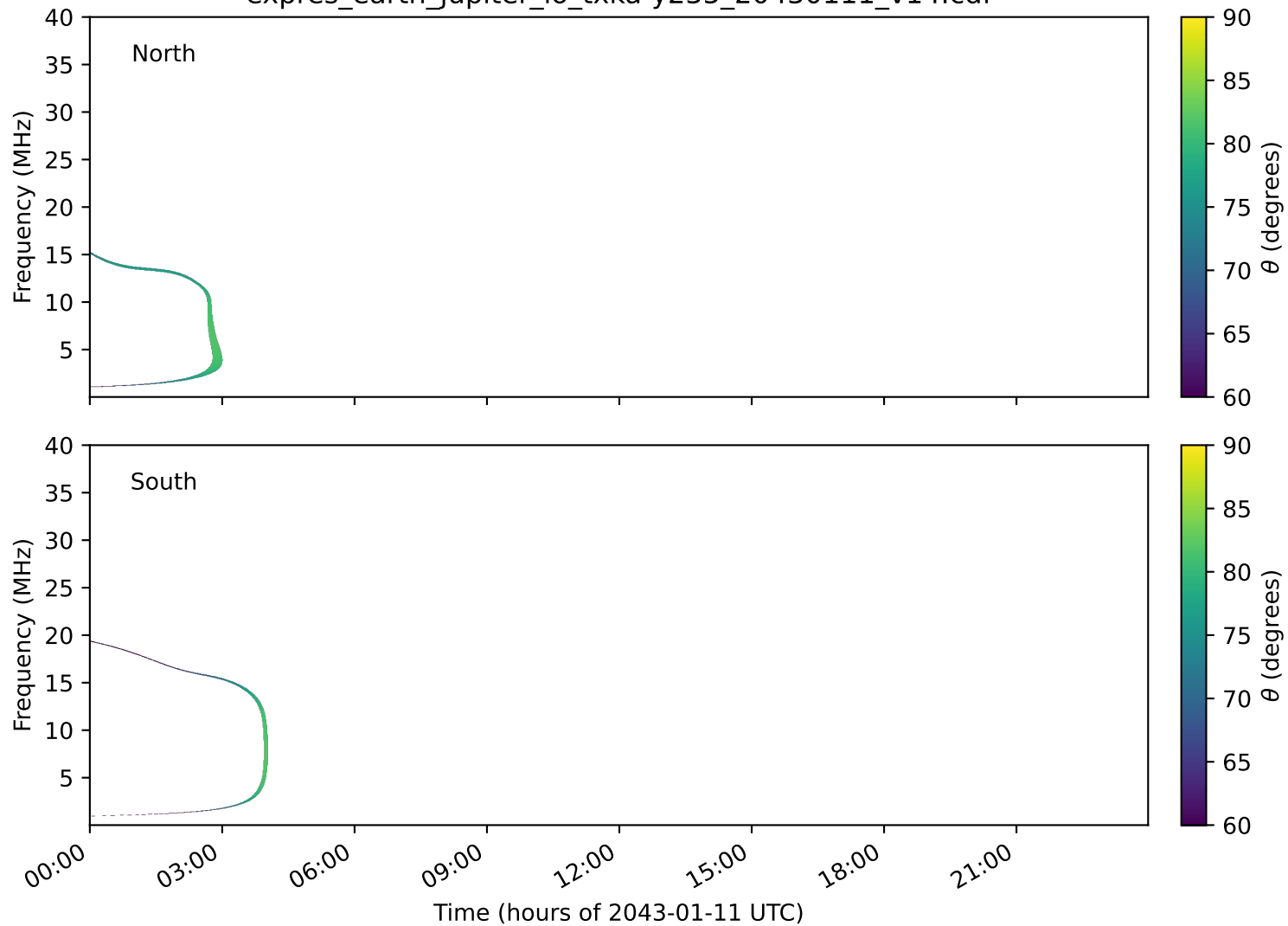
expres_earth_jupiter_io_txka-y235_20430111_v14.cdf
