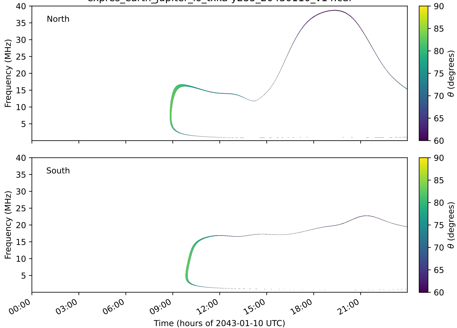
expres_earth_jupiter_io_txka-y235_20430110_v14.cdf
