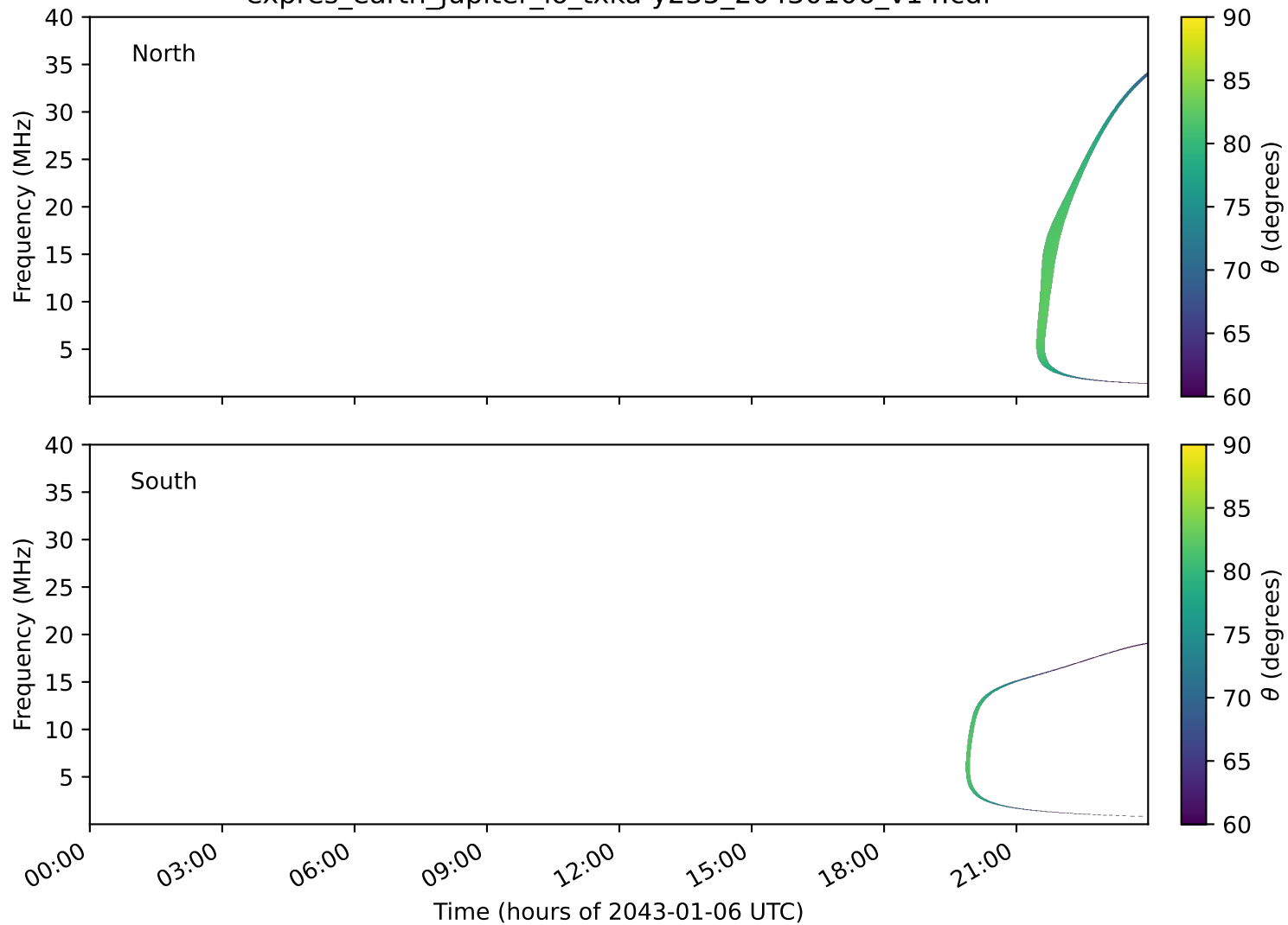
expres_earth_jupiter_io_txka-y235_20430106_v14.cdf
