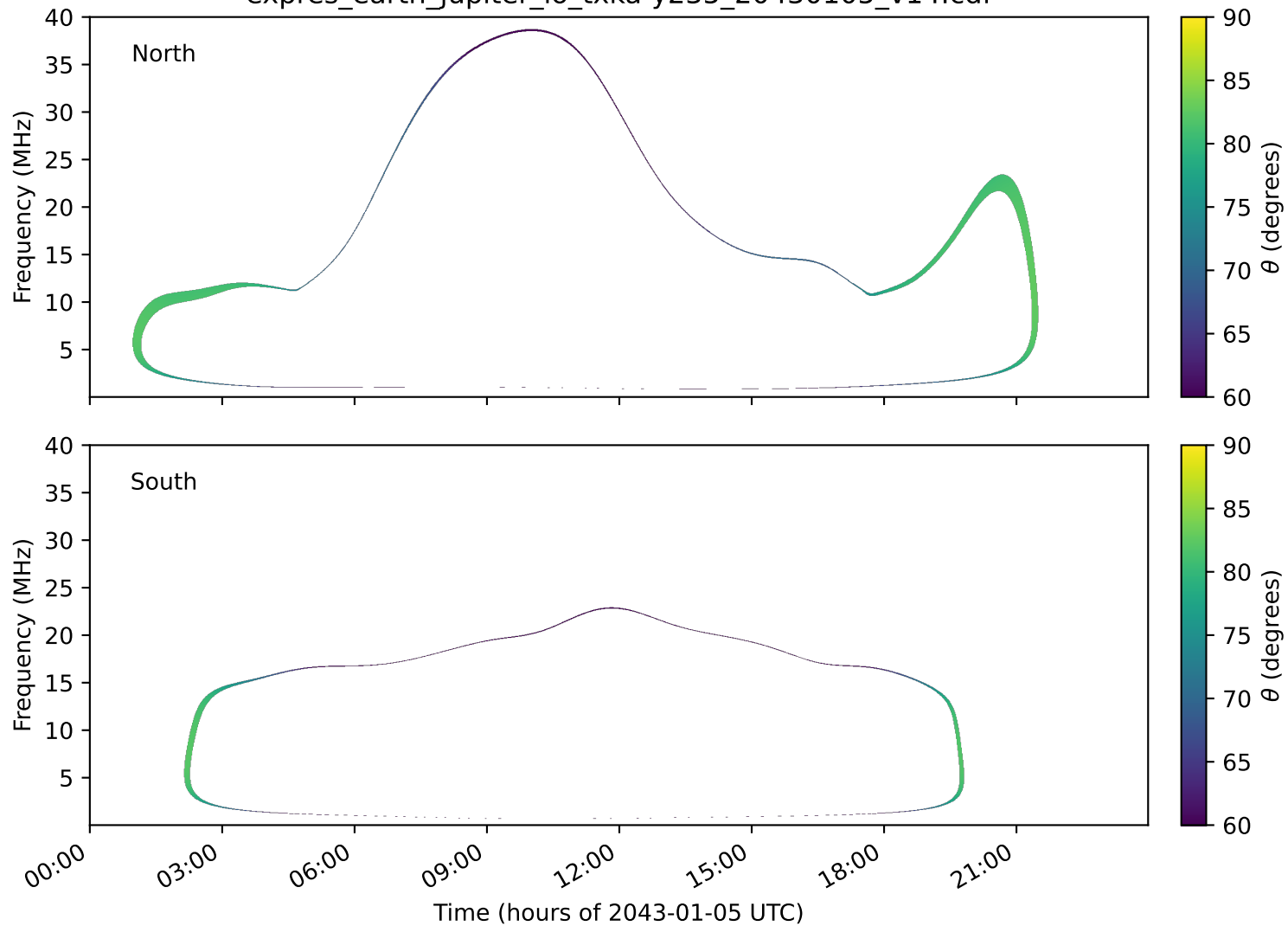
expres_earth_jupiter_io_txka-y235_20430105_v14.cdf
