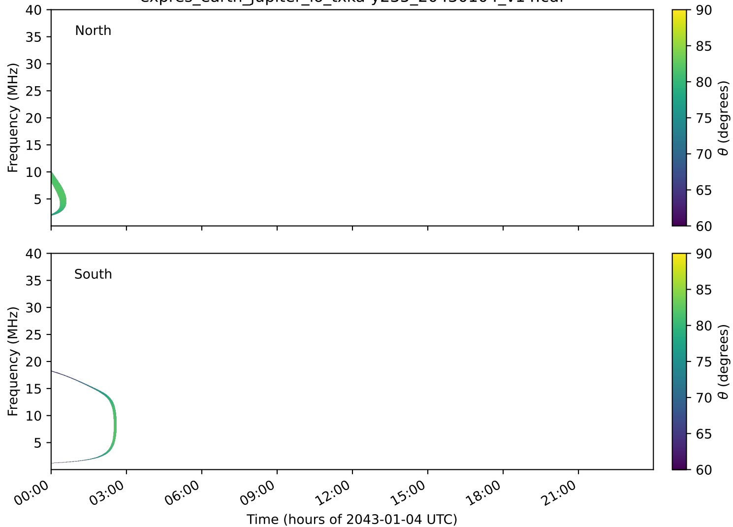
expres_earth_jupiter_io_txka-y235_20430104_v14.cdf
