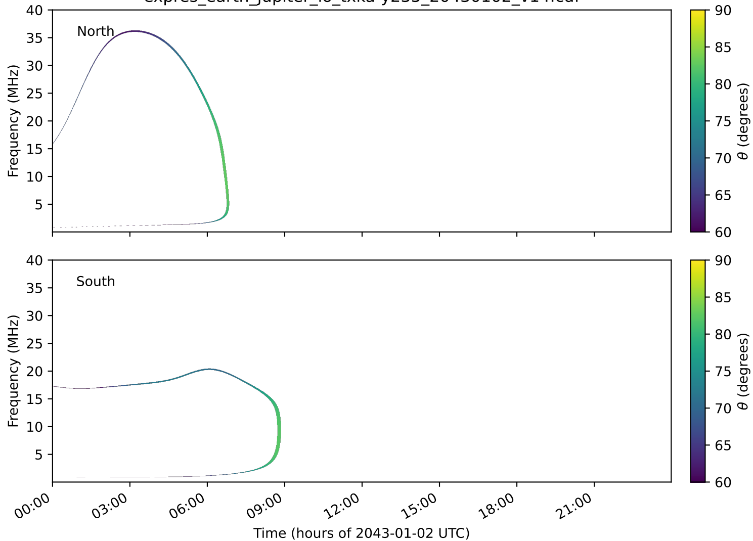
expres_earth_jupiter_io_txka-y235_20430102_v14.cdf
