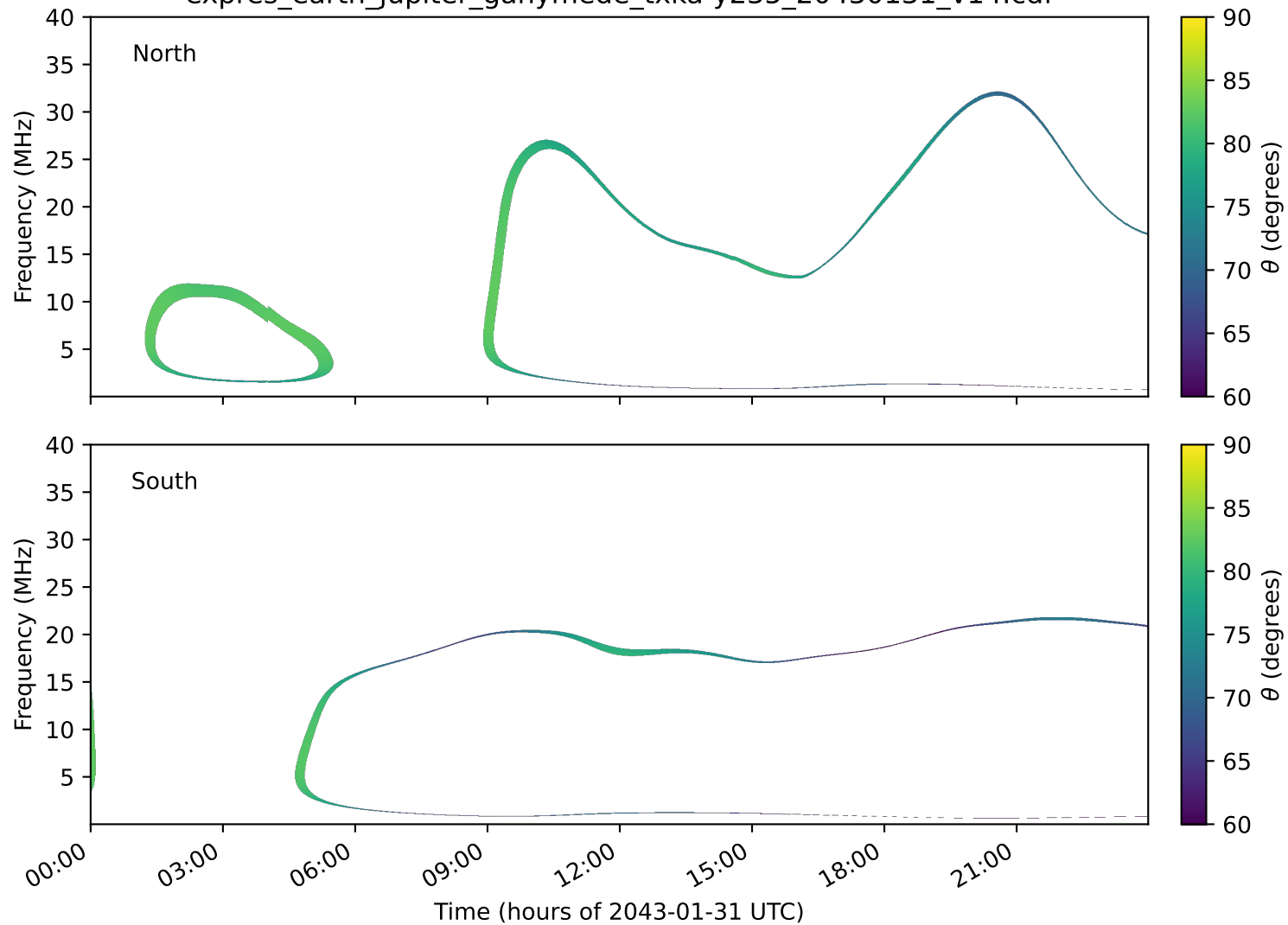
expres_earth_jupiter_ganymede_txka-y235_20430131_v14.cdf
