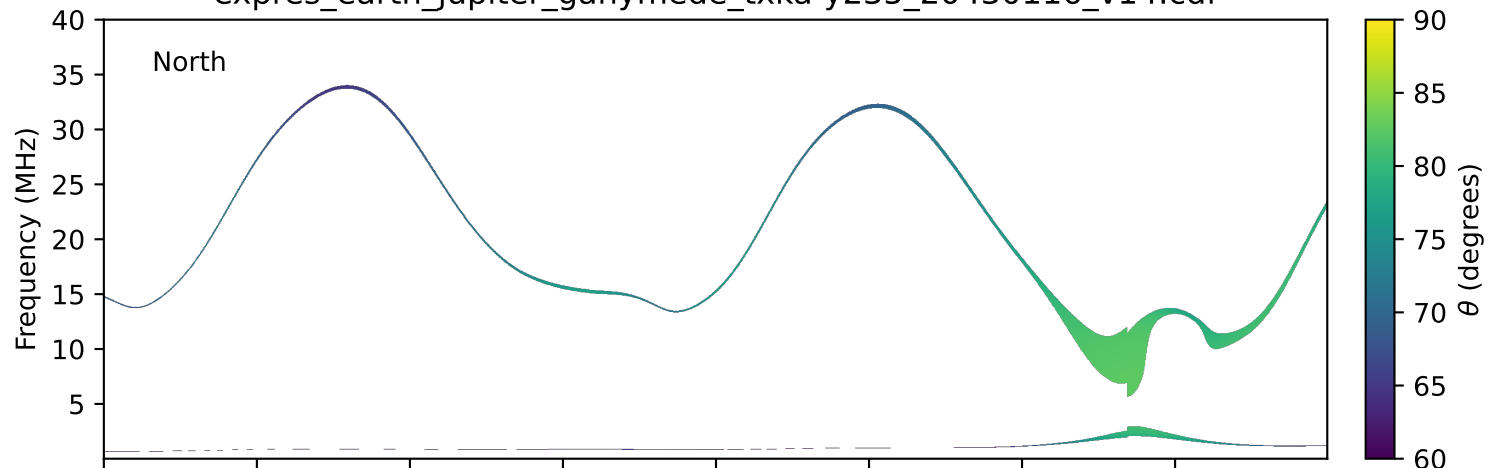
expres_earth_jupiter_ganymede_txka-y235_20430116_v14.cdf
