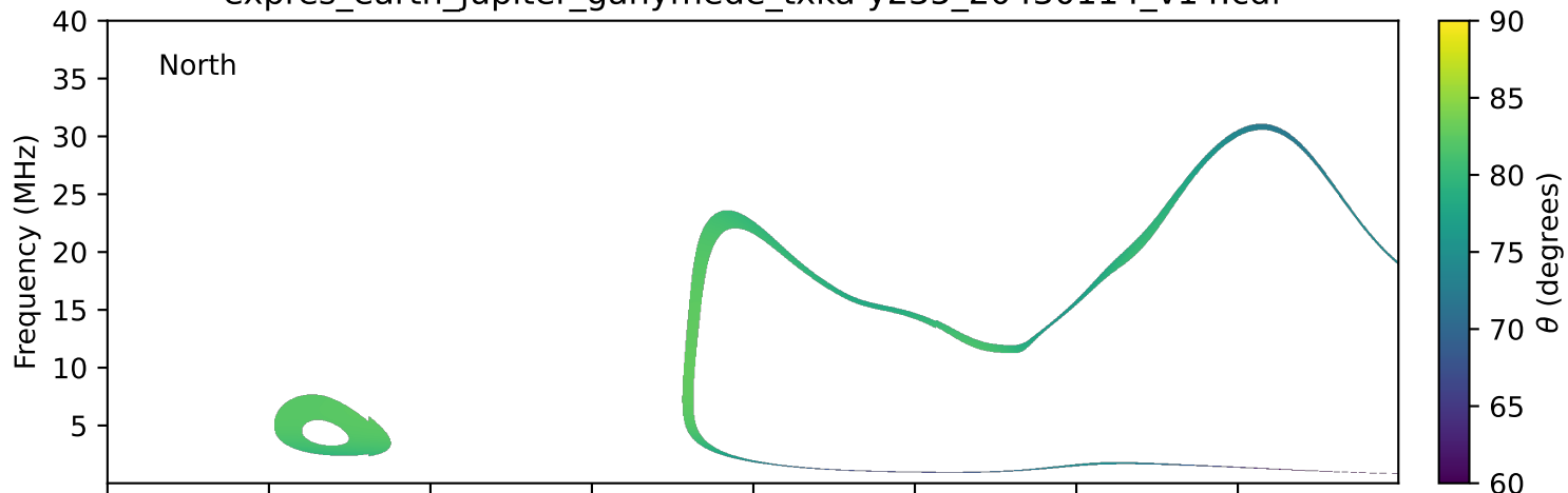
expres_earth_jupiter_ganymede_txka-y235_20430114_v14.cdf
