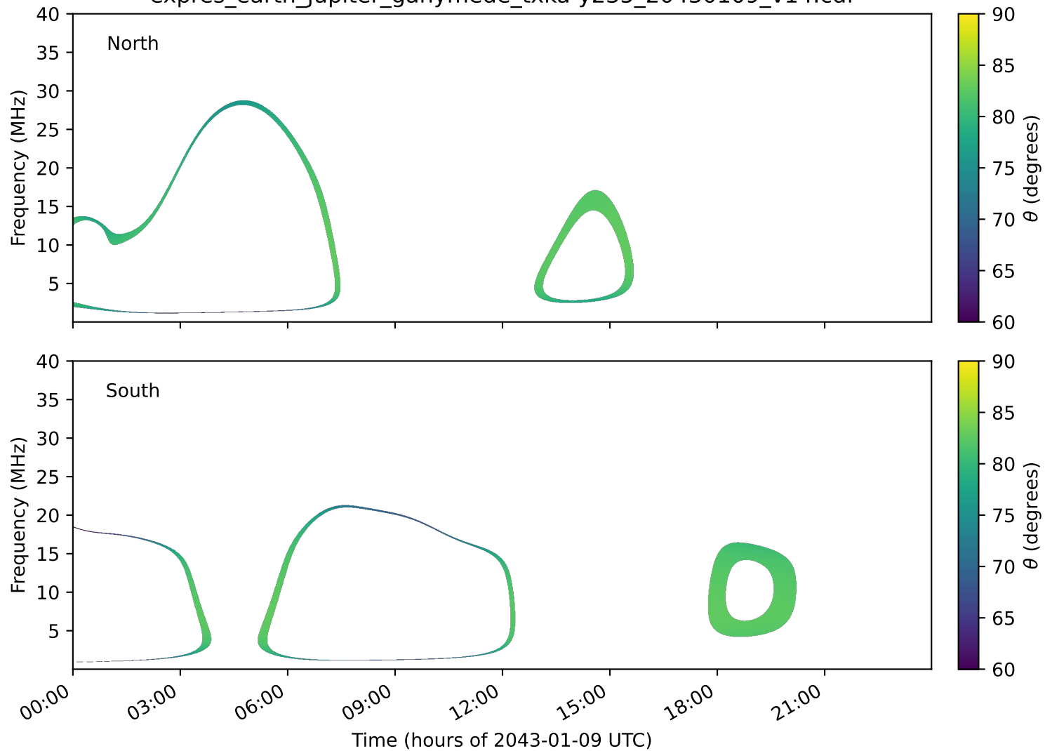
expres_earth_jupiter_ganymede_txka-y235_20430109_v14.cdf
