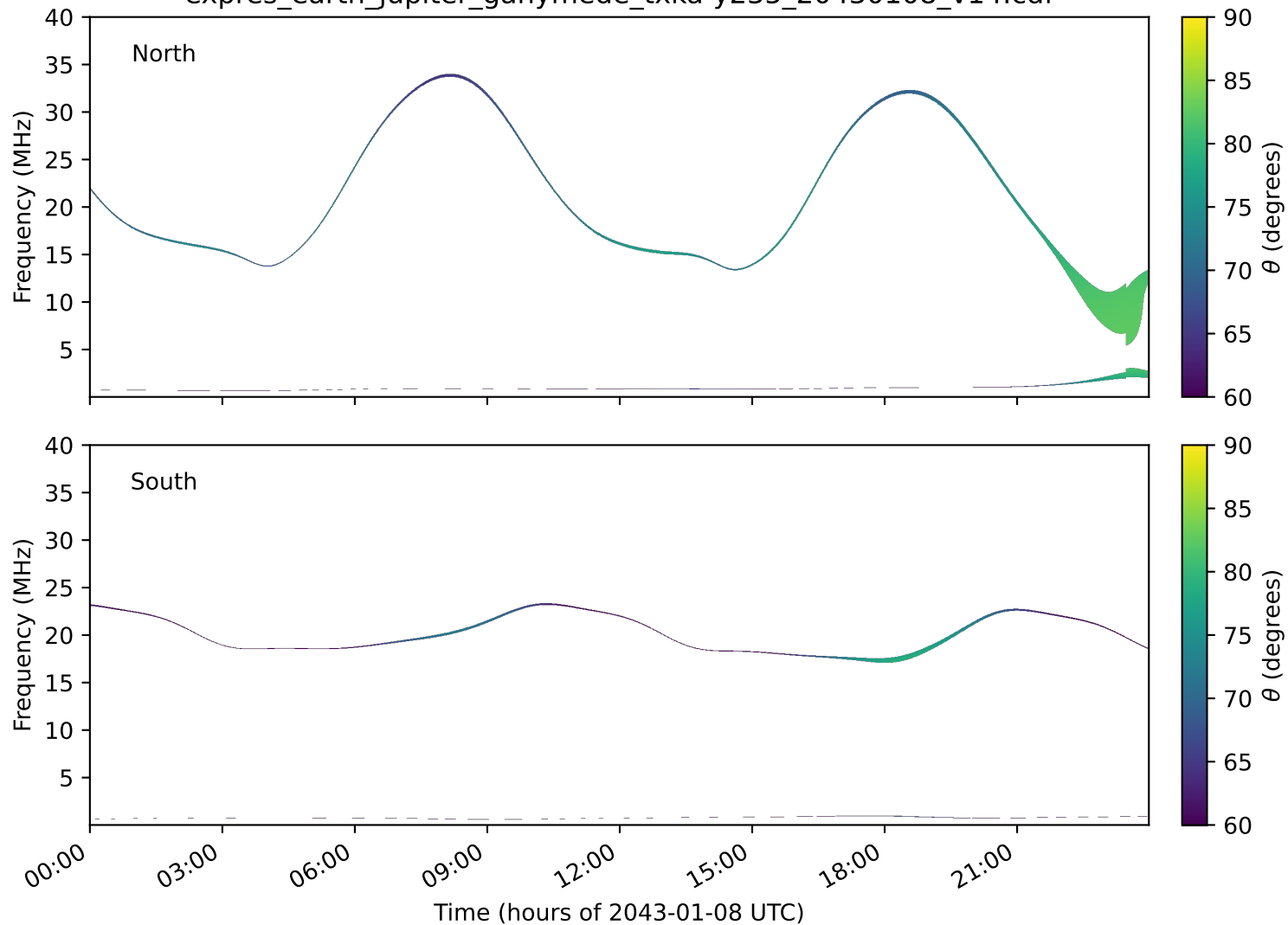
expres_earth_jupiter_ganymede_txka-y235_20430108_v14.cdf
