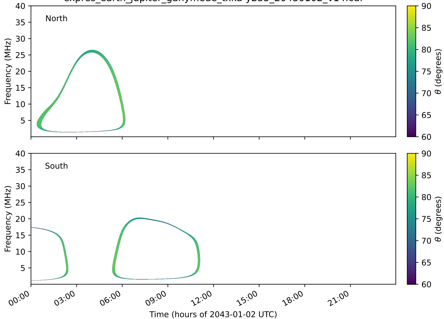
expres_earth_jupiter_ganymede_txka-y235_20430102_v14.cdf
