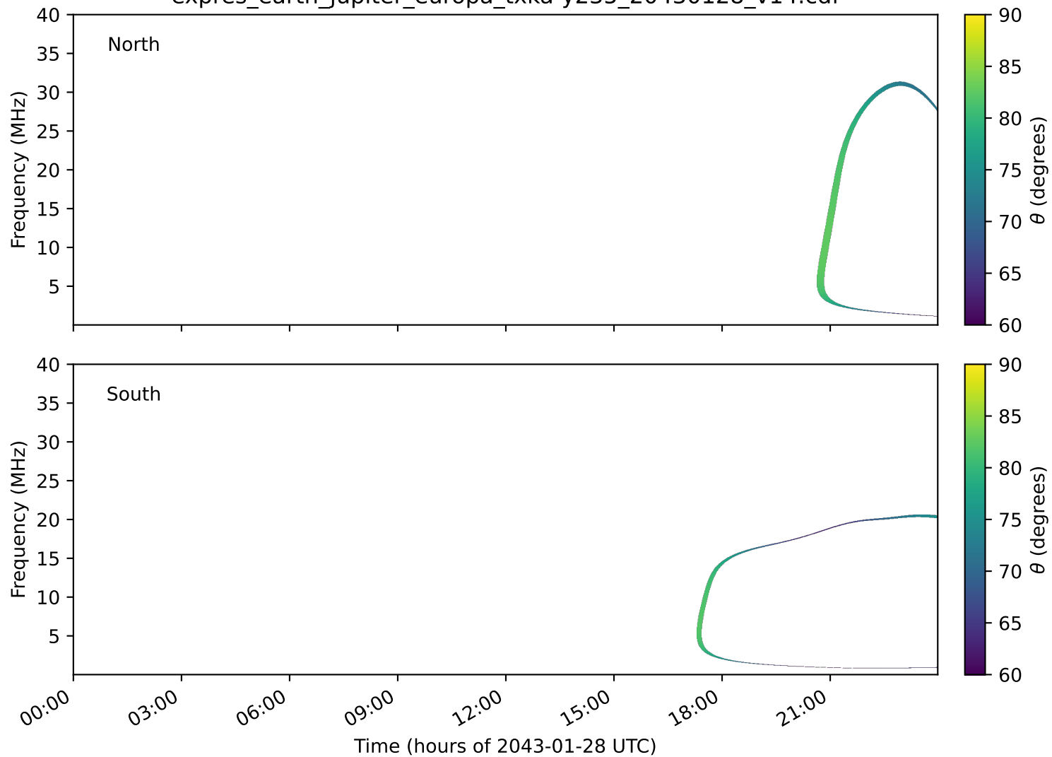
expres_earth_jupiter_europa_txka-y235_20430128_v14.cdf
