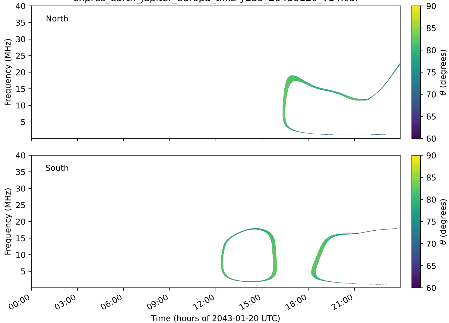
expres_earth_jupiter_europa_txka-y235_20430120_v14.cdf
