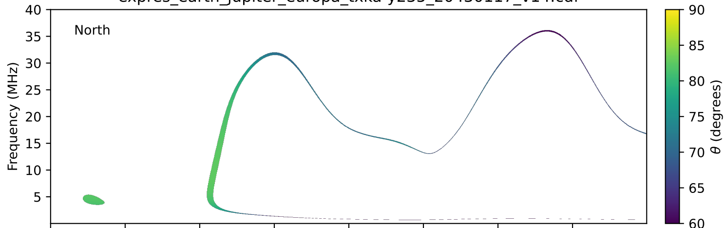
expres_earth_jupiter_europa_txka-y235_20430117_v14.cdf
