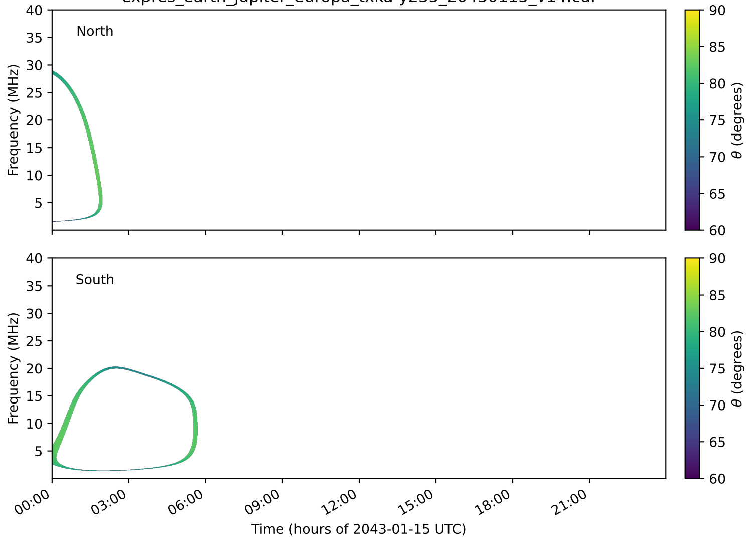
expres_earth_jupiter_europa_txka-y235_20430115_v14.cdf
