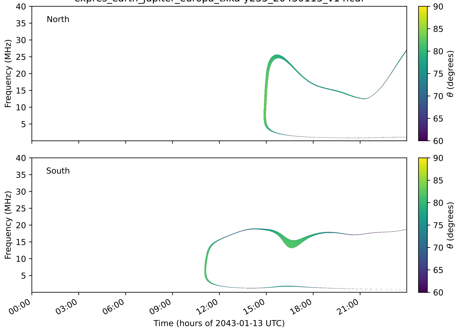
expres_earth_jupiter_europa_txka-y235_20430113_v14.cdf
