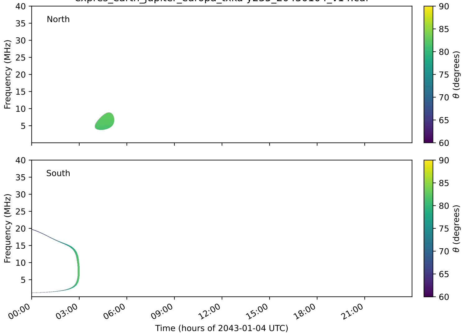
expres_earth_jupiter_europa_txka-y235_20430104_v14.cdf
