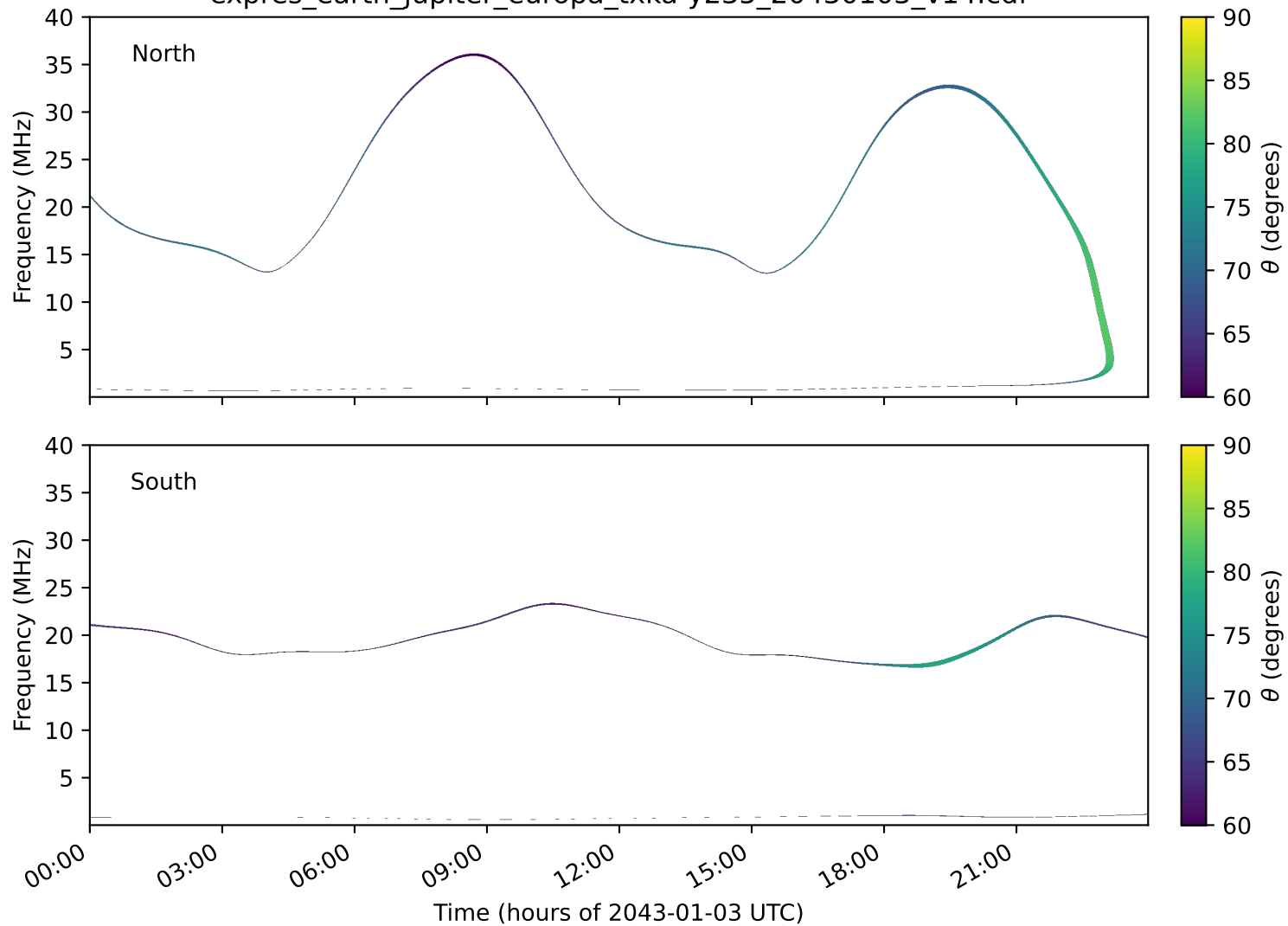
expres_earth_jupiter_europa_txka-y235_20430103_v14.cdf
