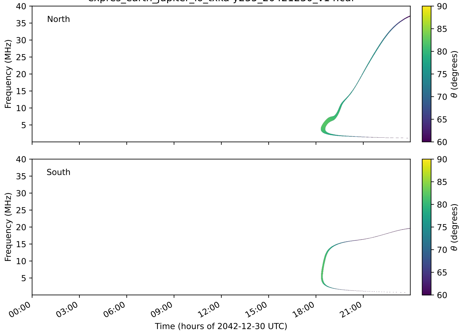
expres_earth_jupiter_io_txka-y235_20421230_v14.cdf
