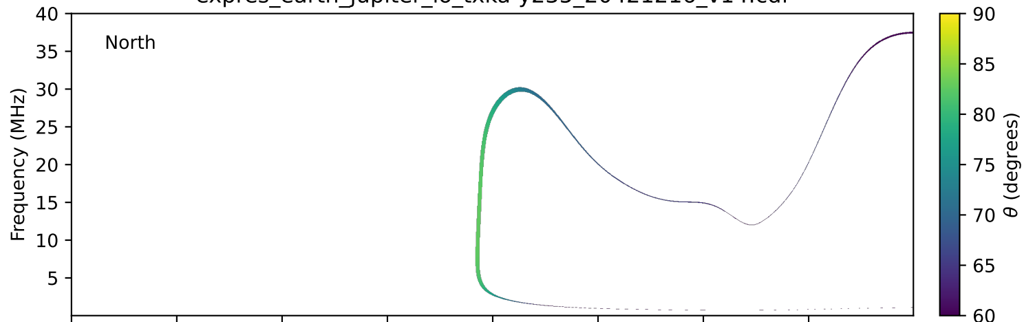
expres_earth_jupiter_io_txka-y235_20421216_v14.cdf
