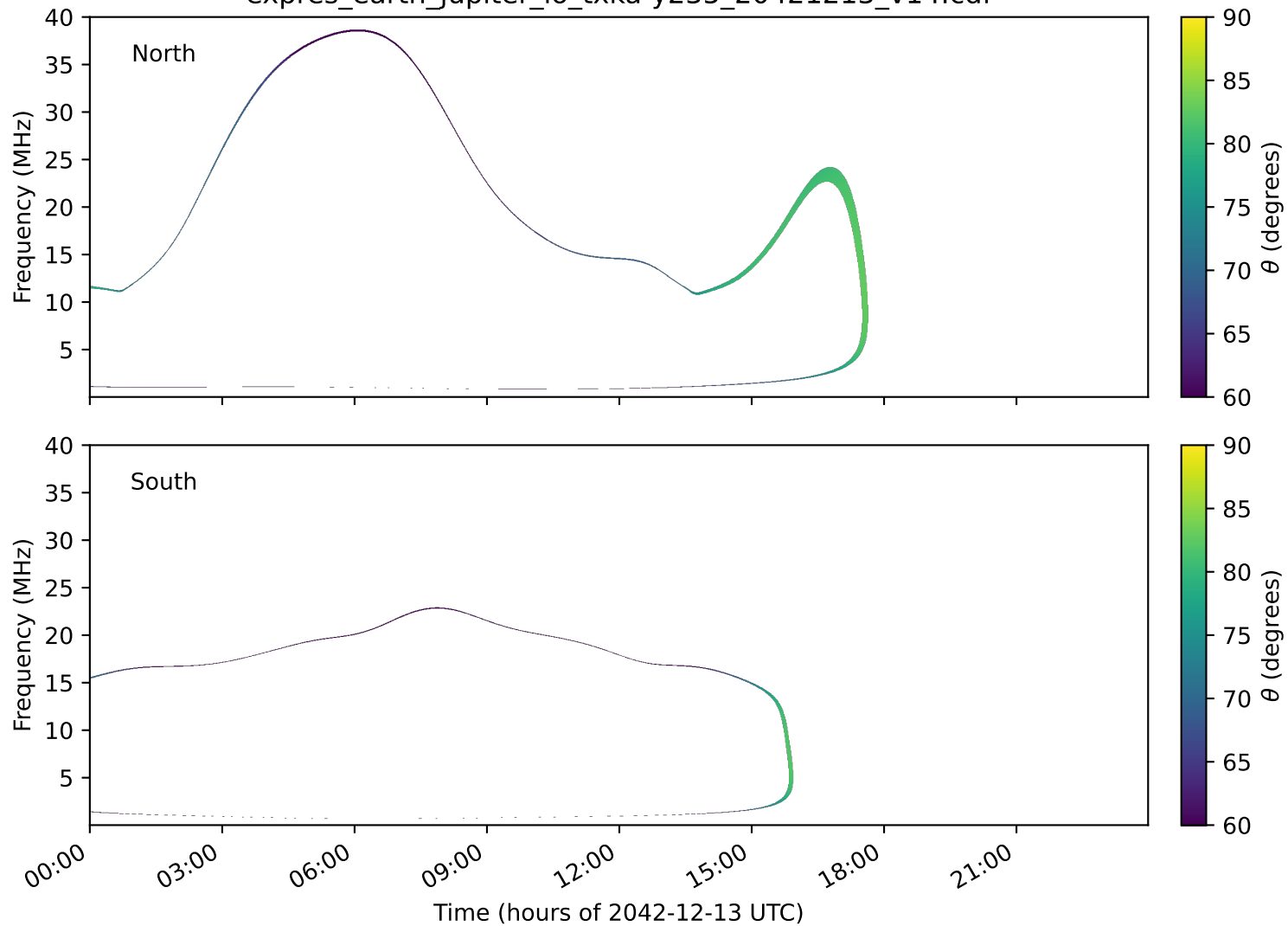
expres_earth_jupiter_io_txka-y235_20421213_v14.cdf
