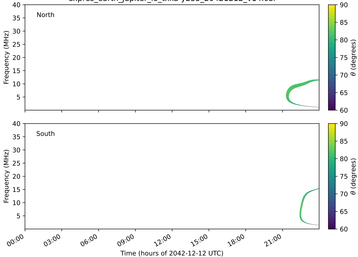
expres_earth_jupiter_io_txka-y235_20421212_v14.cdf
