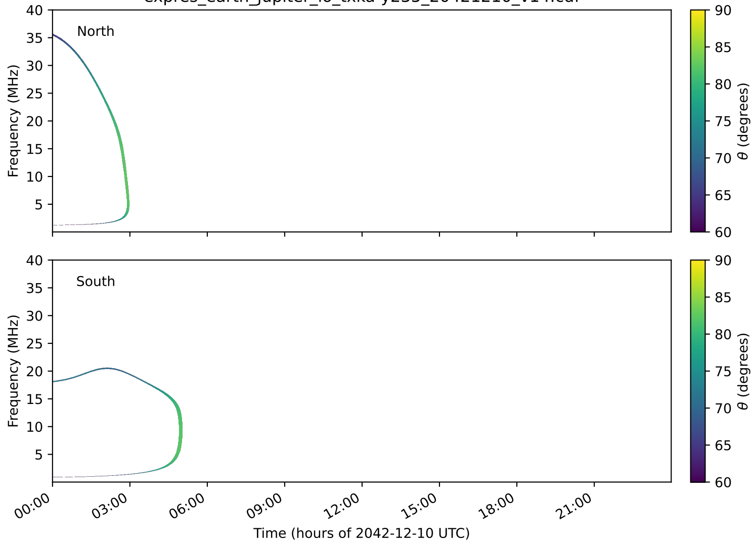
expres_earth_jupiter_io_txka-y235_20421210_v14.cdf
