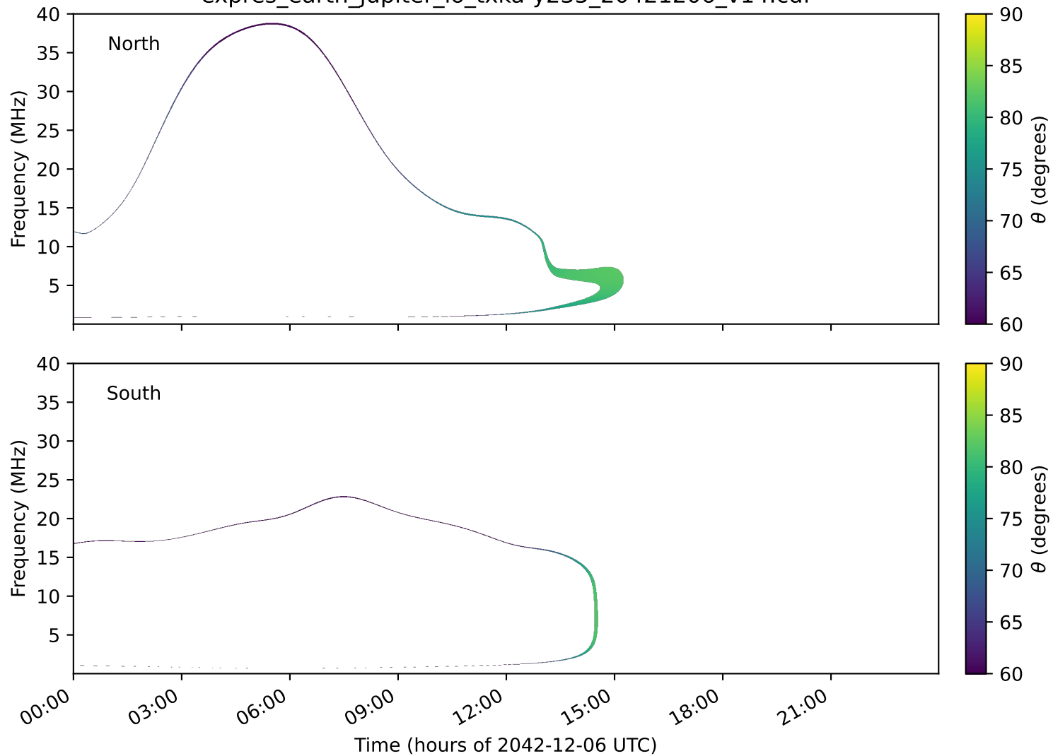
expres_earth_jupiter_io_txka-y235_20421206_v14.cdf
