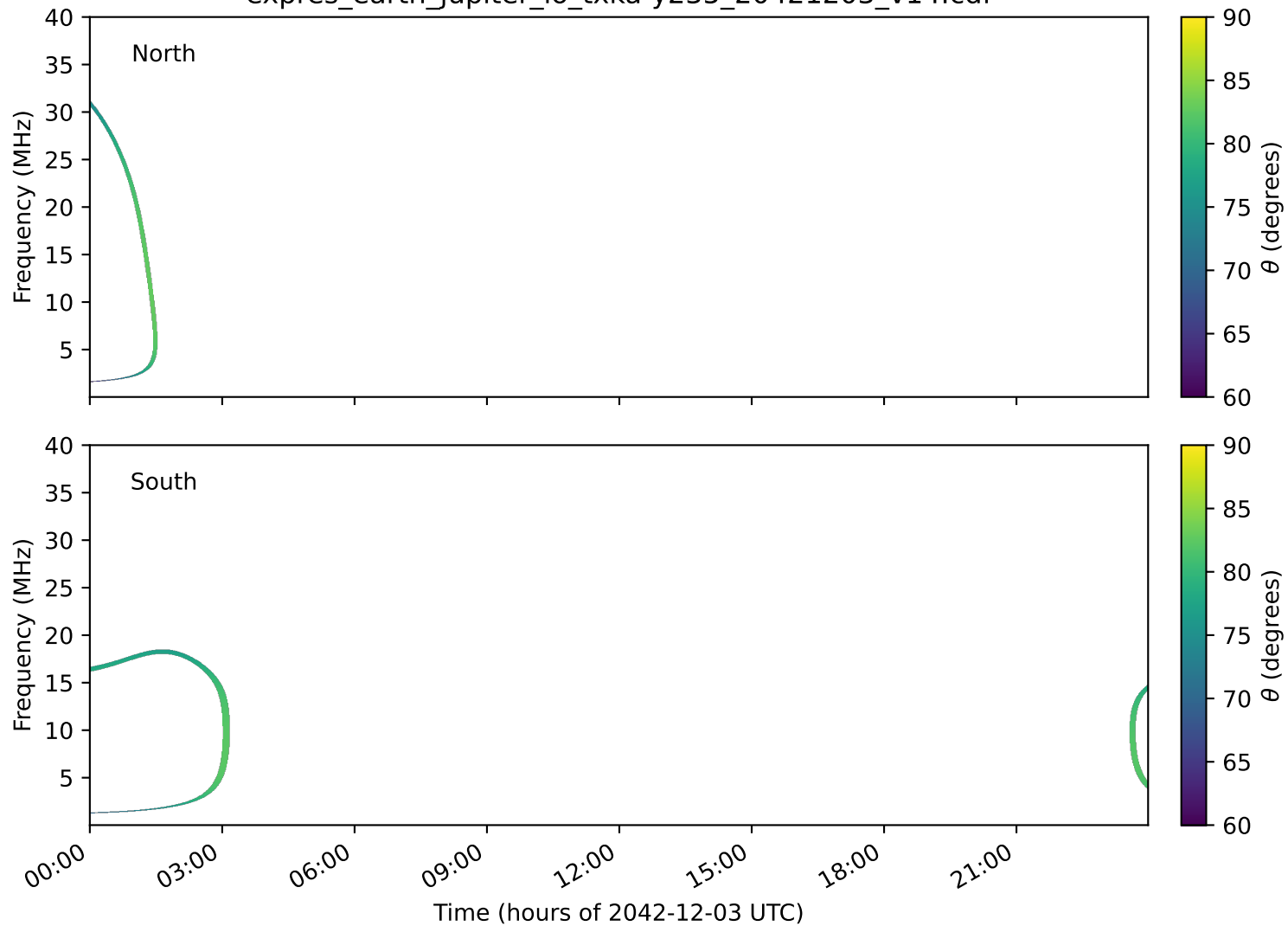
expres_earth_jupiter_io_txka-y235_20421203_v14.cdf
