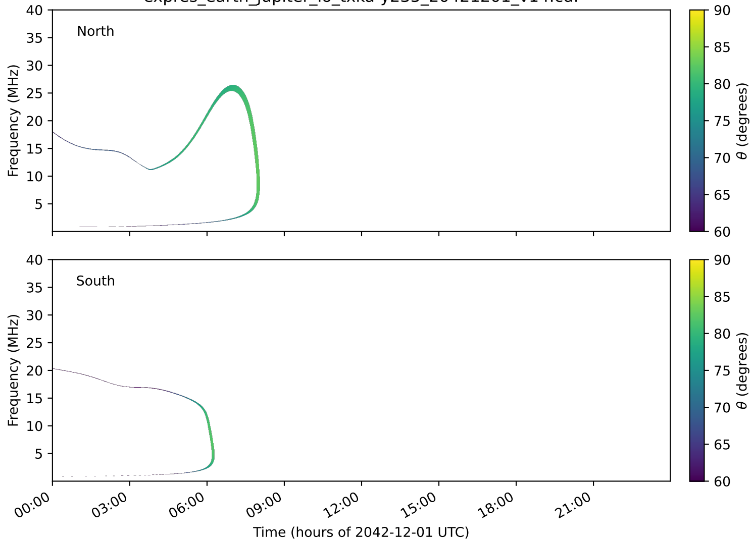
expres_earth_jupiter_io_txka-y235_20421201_v14.cdf
