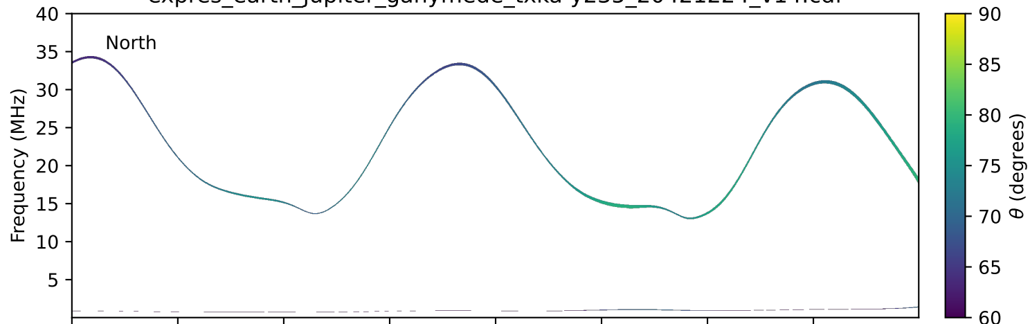
expres_earth_jupiter_ganymede_txka-y235_20421224_v14.cdf
