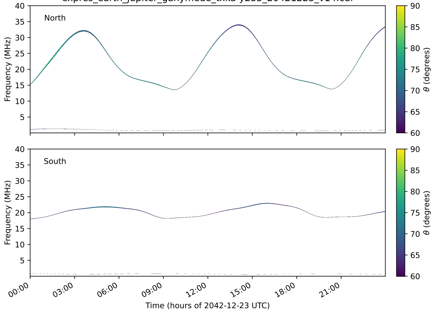
expres_earth_jupiter_ganymede_txka-y235_20421223_v14.cdf
