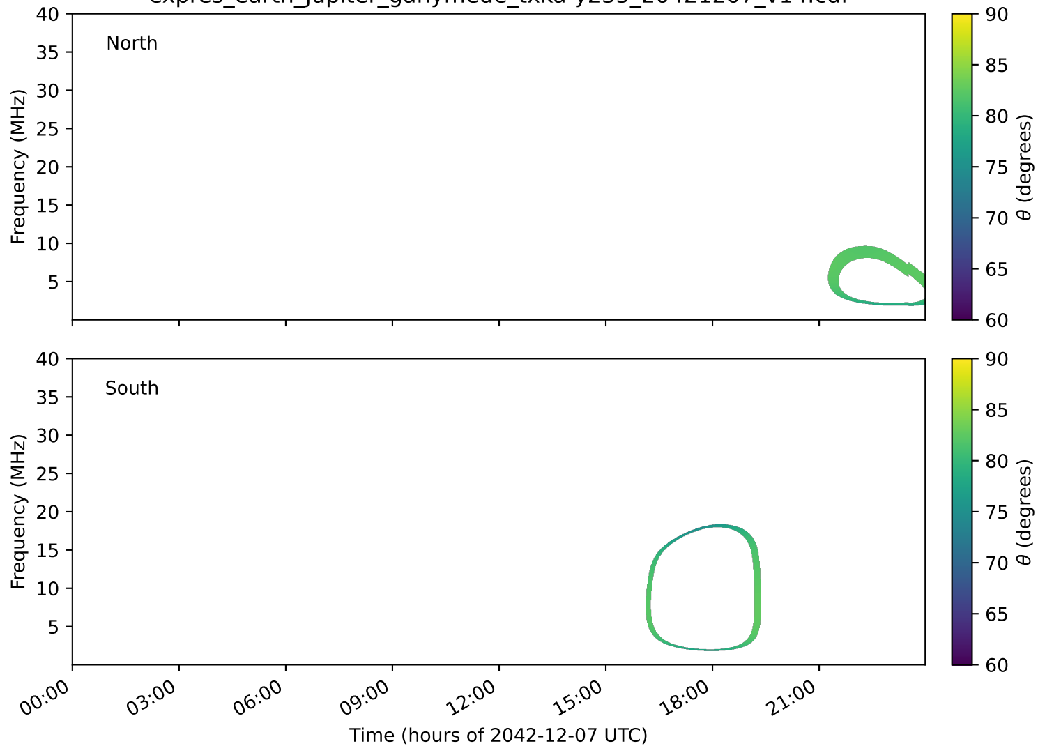
expres_earth_jupiter_ganymede_txka-y235_20421207_v14.cdf
