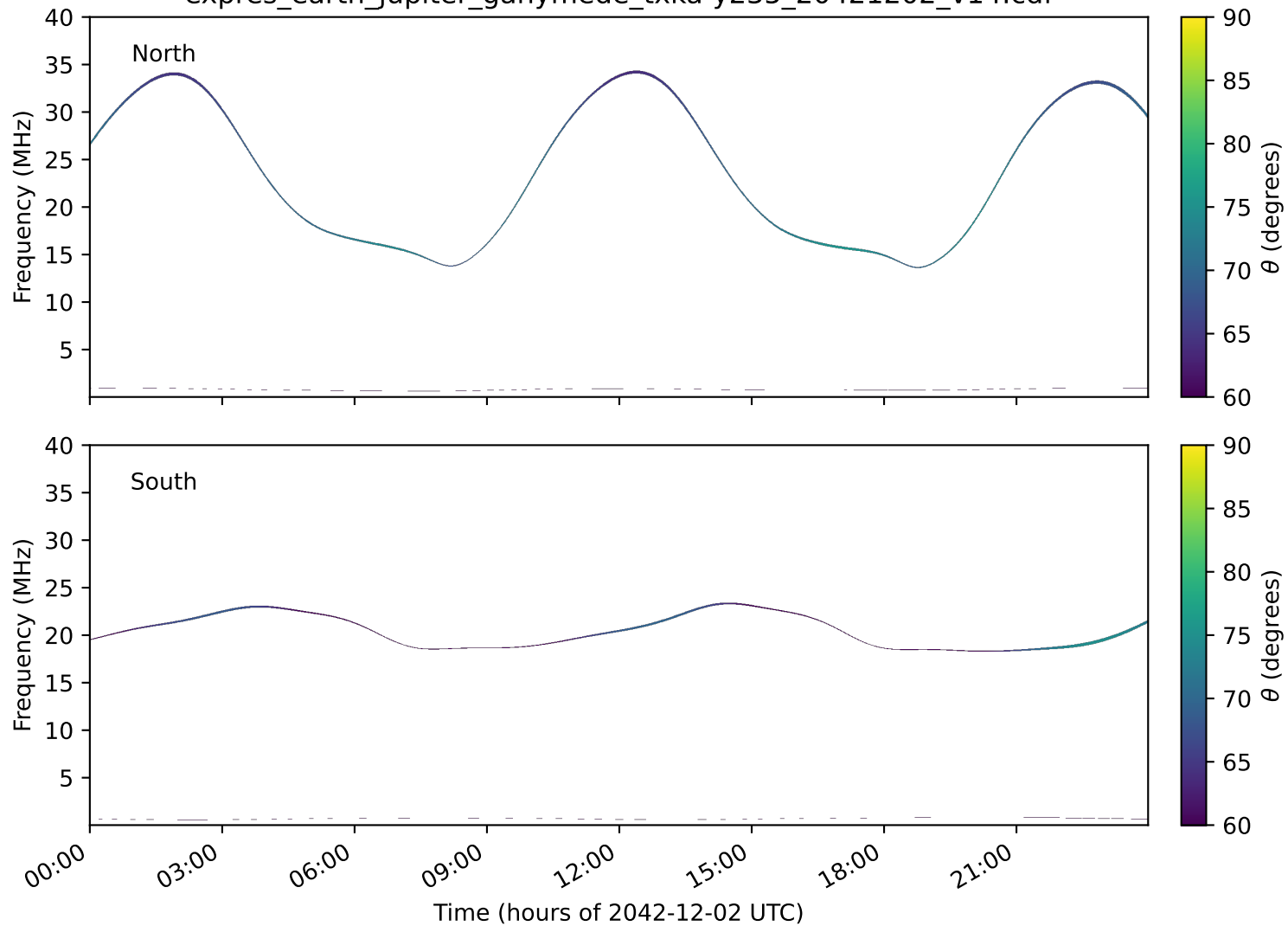
expres_earth_jupiter_ganymede_txka-y235_20421202_v14.cdf
