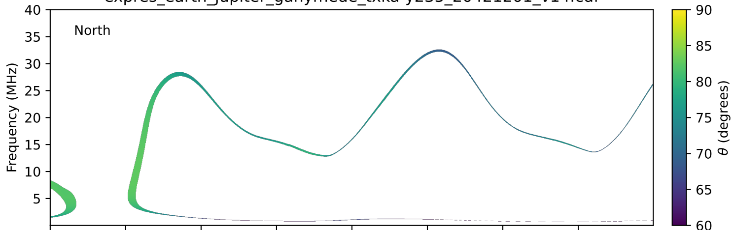
expres_earth_jupiter_ganymede_txka-y235_20421201_v14.cdf
