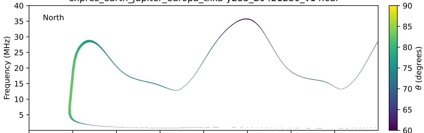
expres_earth_jupiter_europa_txka-y235_20421230_v14.cdf
