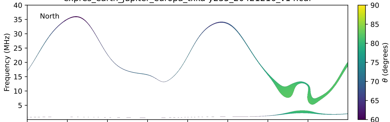
expres_earth_jupiter_europa_txka-y235_20421216_v14.cdf
