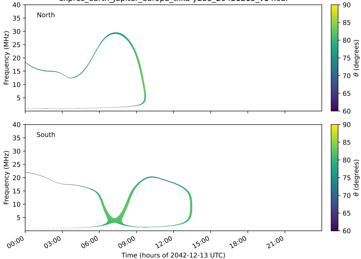
expres_earth_jupiter_europa_txka-y235_20421213_v14.cdf
