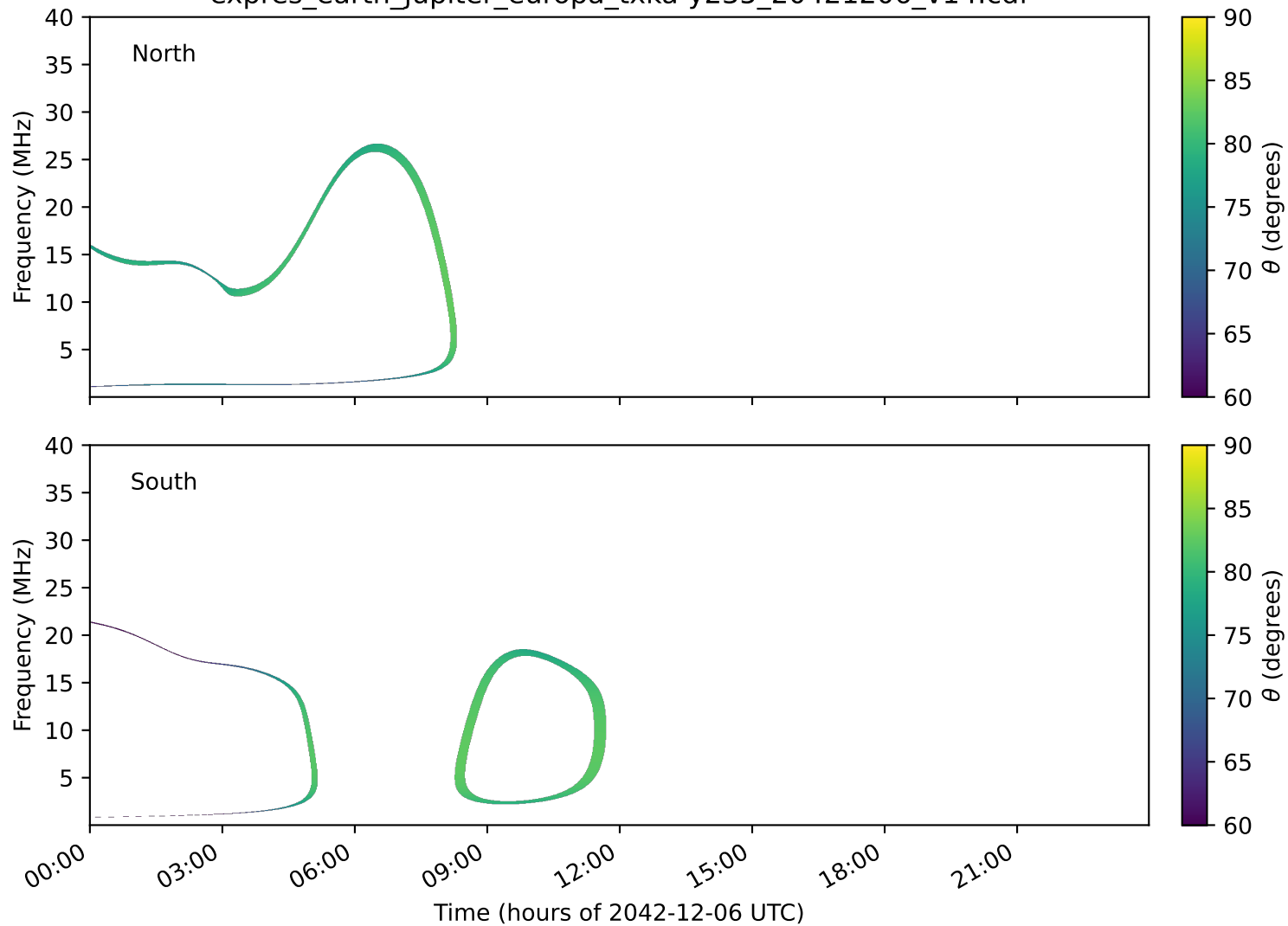
expres_earth_jupiter_europa_txka-y235_20421206_v14.cdf
