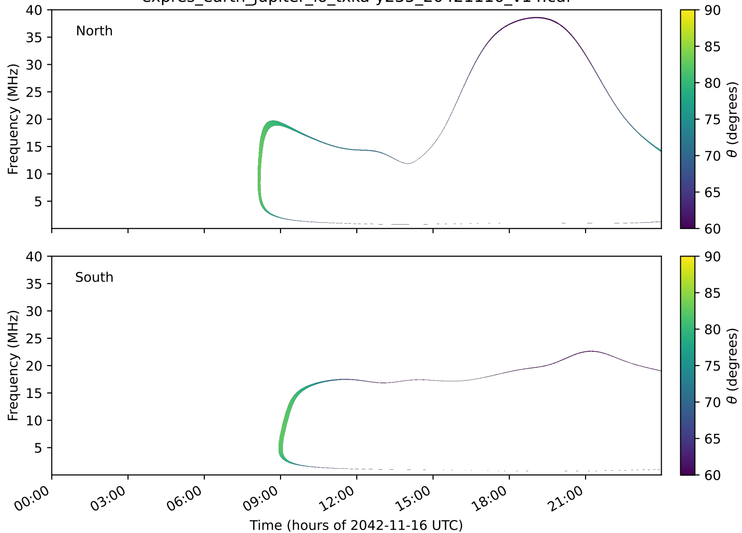
expres_earth_jupiter_io_txka-y235_20421116_v14.cdf
