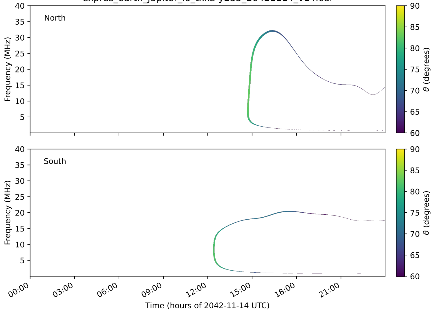
expres_earth_jupiter_io_txka-y235_20421114_v14.cdf
