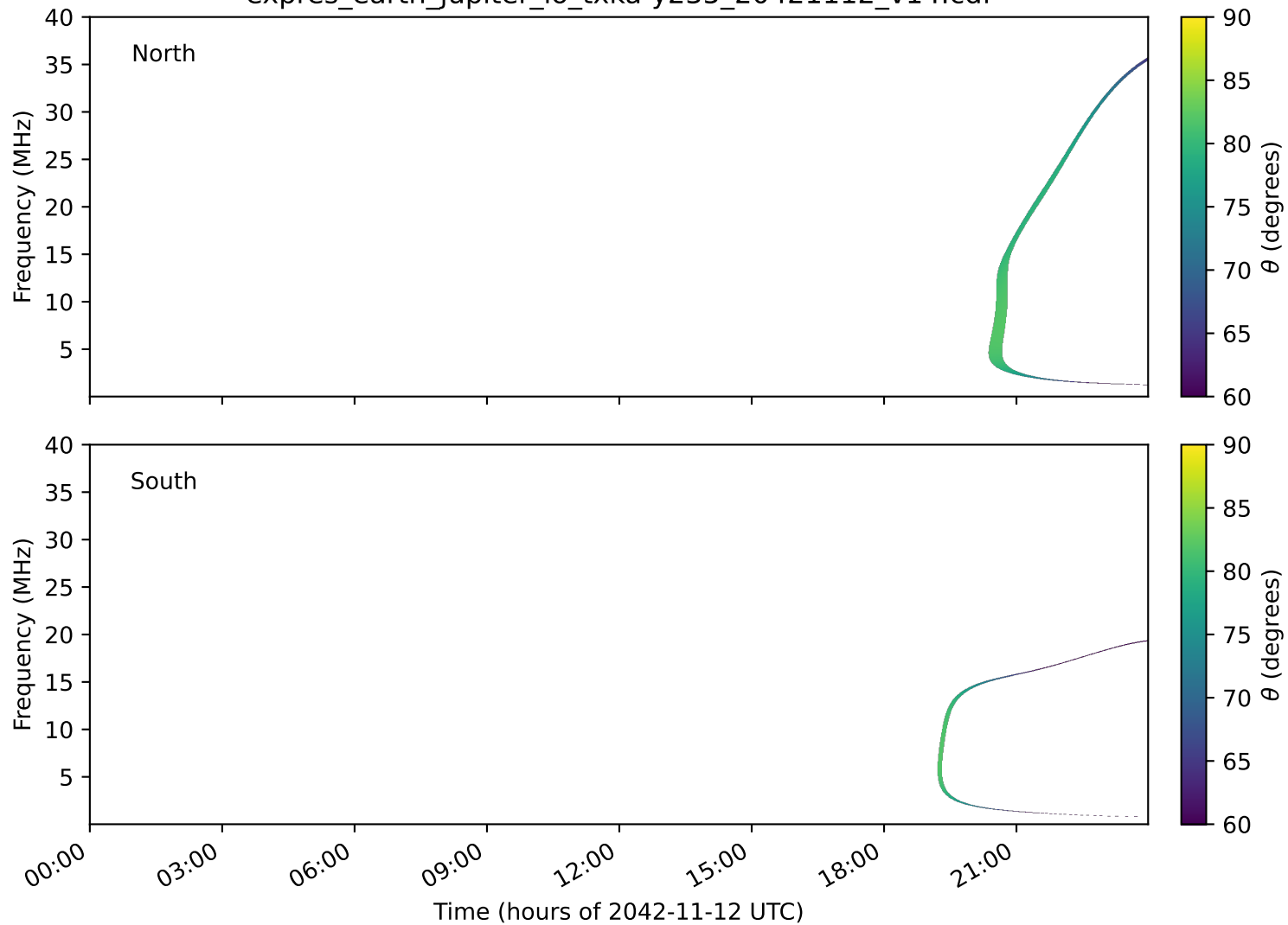
expres_earth_jupiter_io_txka-y235_20421112_v14.cdf
