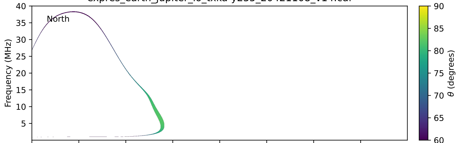
expres_earth_jupiter_io_txka-y235_20421108_v14.cdf
