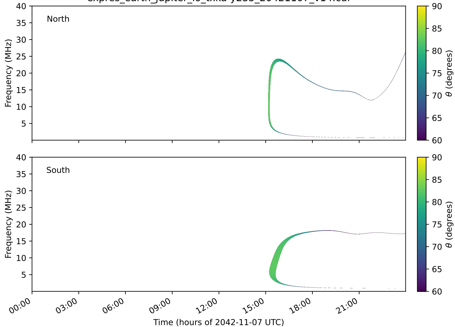
expres_earth_jupiter_io_txka-y235_20421107_v14.cdf
