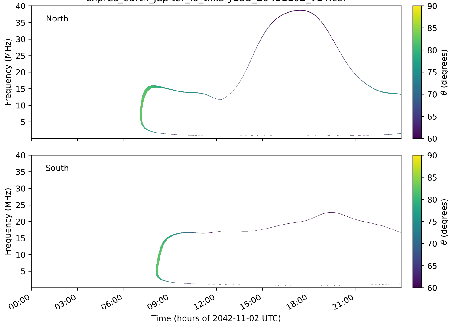
expres_earth_jupiter_io_txka-y235_20421102_v14.cdf
