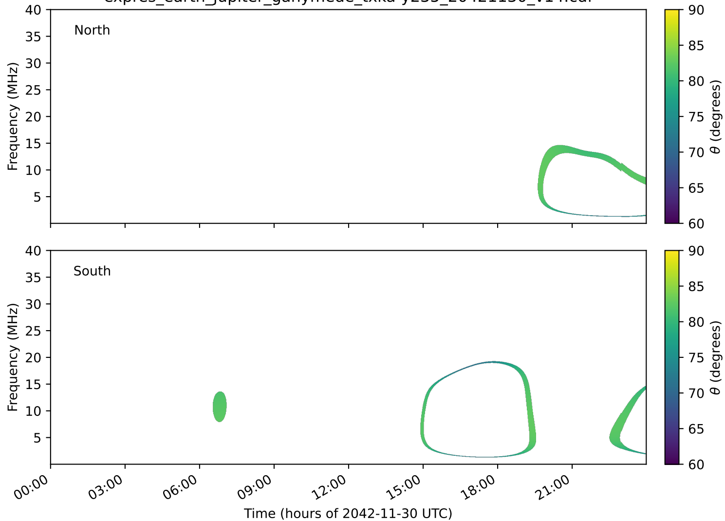
expres_earth_jupiter_ganymede_txka-y235_20421130_v14.cdf
