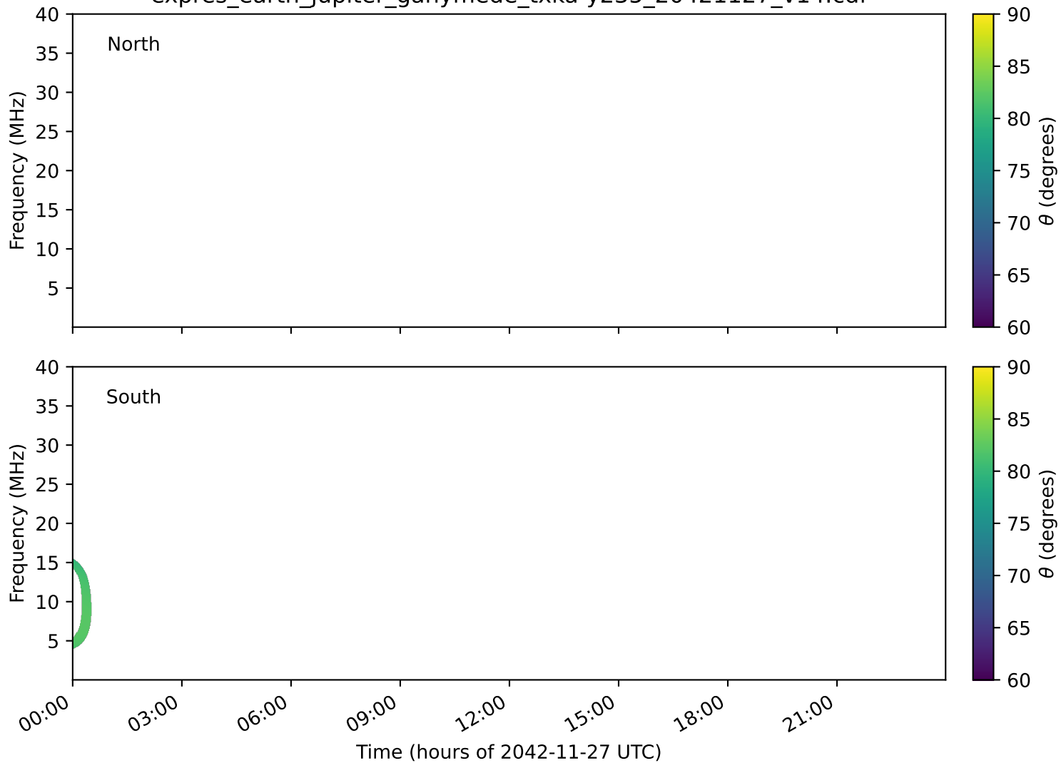
expres_earth_jupiter_ganymede_txka-y235_20421127_v14.cdf
