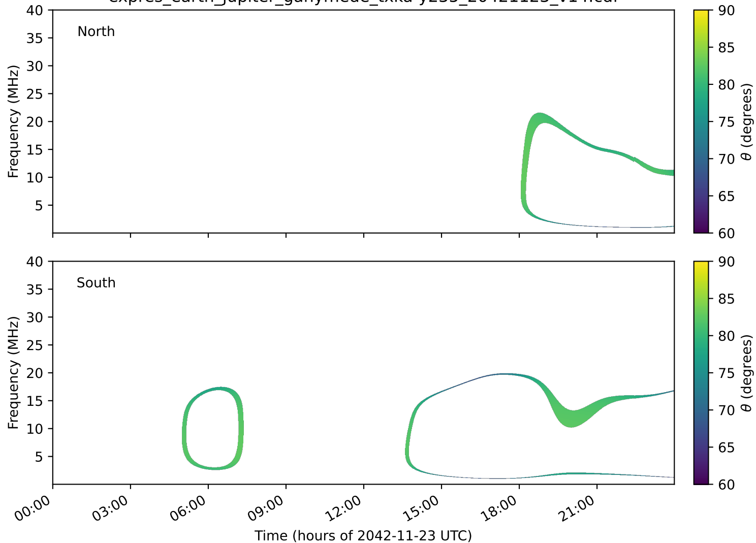
expres_earth_jupiter_ganymede_txka-y235_20421123_v14.cdf
