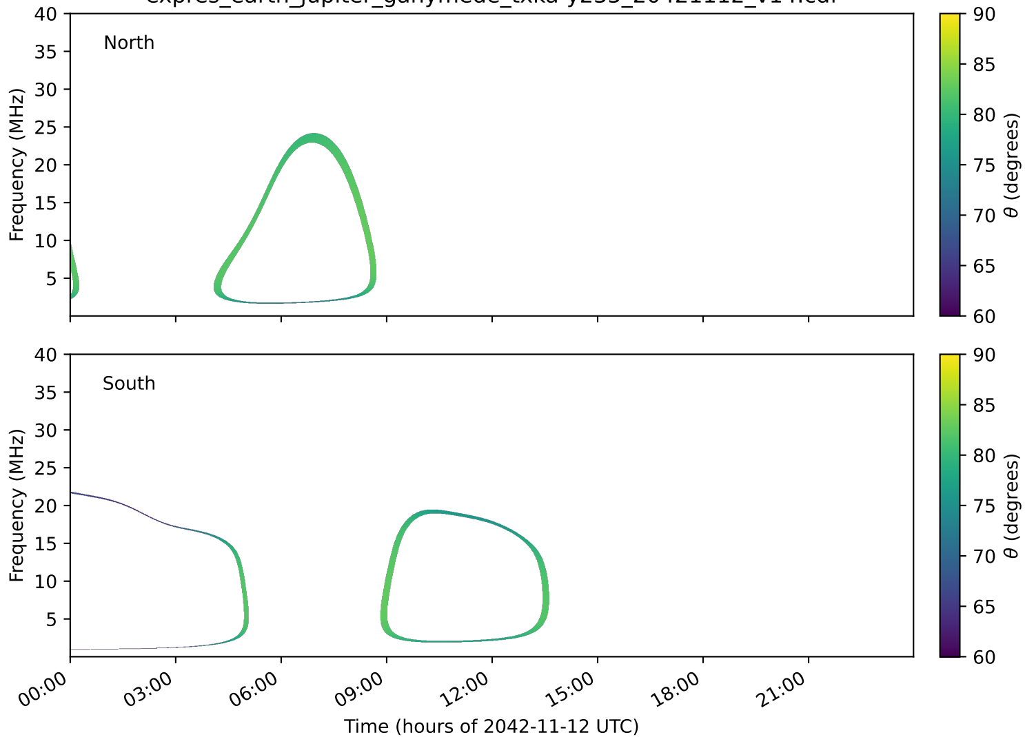
expres_earth_jupiter_ganymede_txka-y235_20421112_v14.cdf
