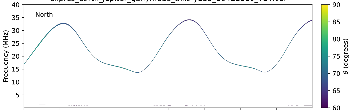
expres_earth_jupiter_ganymede_txka-y235_20421110_v14.cdf
