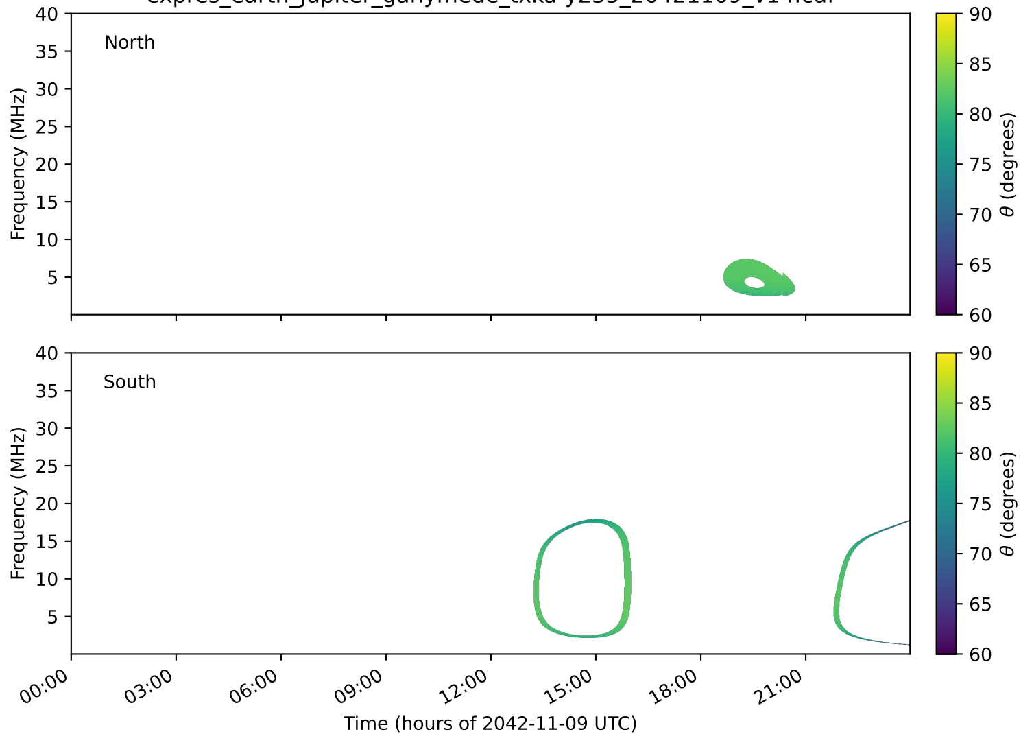
expres_earth_jupiter_ganymede_txka-y235_20421109_v14.cdf
